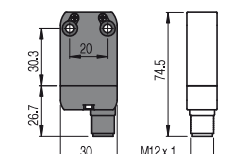
M12 connector, bottom
